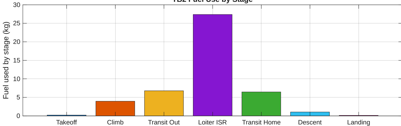
TB2 Fuel Use by Stage
