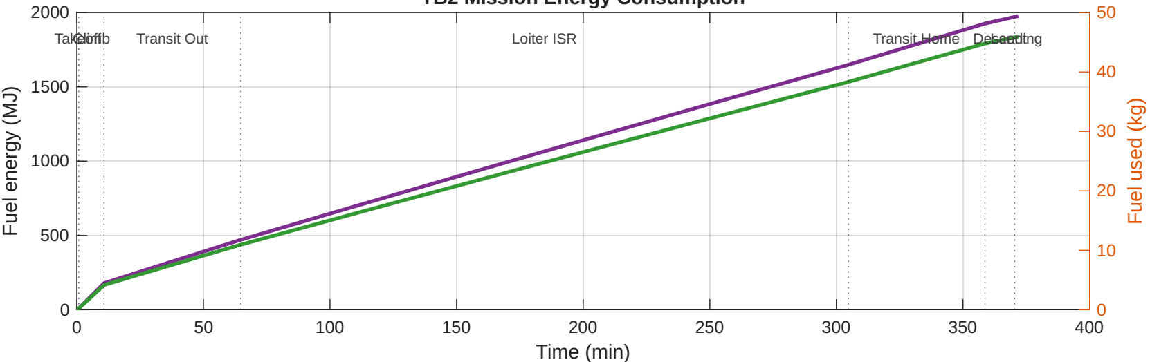
TB2 Mission Energy Consumption
